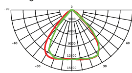
Light Distribution Curve
